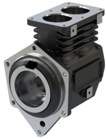
697.01.1100 Crankcase
