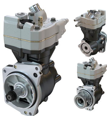
832.01.2000 (WITH GEAR)
